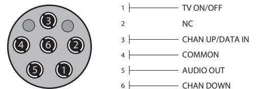
TV Pillow Speaker Interface Pinout
